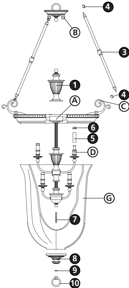
Drawing 1 - Fixture Assembly
