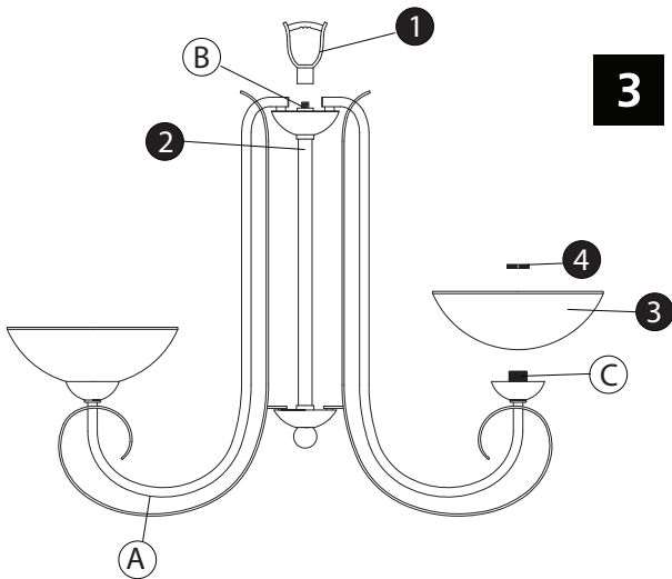
Drawing 1 - Fixture Assembly
