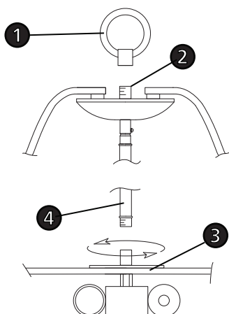
Drawing 1 - Fixture Assembly
