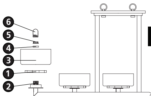
Drawing 1 - Glass Installation
