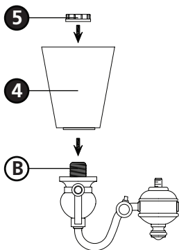
Drawing 2 - Glass Installation
