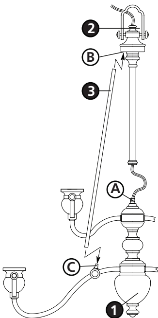
Drawing 1 - Fixture Assembly
