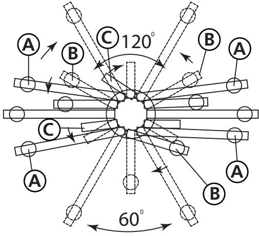
Drawing 1 - Strap Detail
