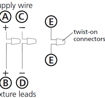
Drawing 3 – Post-Mount
