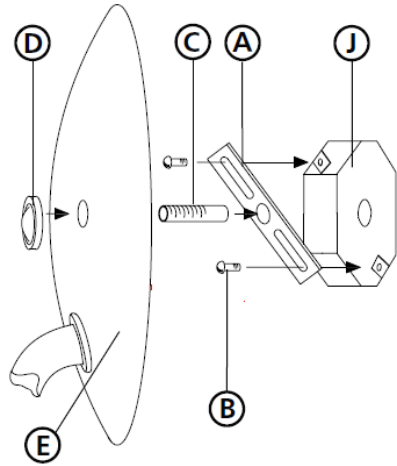
Drawing 2 – Final Assembly
