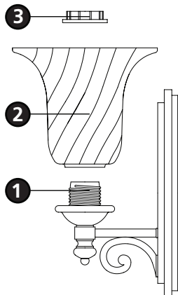
Drawing 3 - Glass Installation
