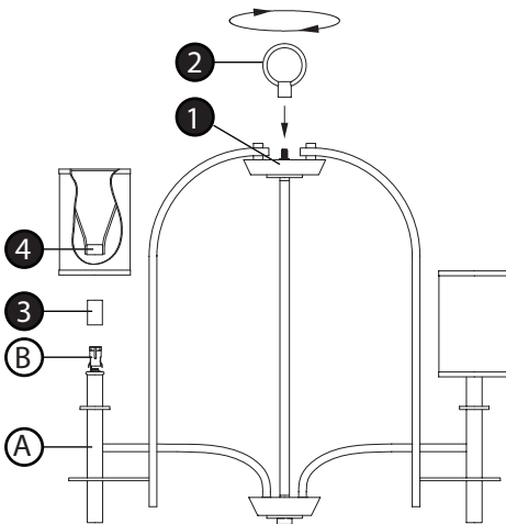
Drawing 2 - Fixture Assembly
