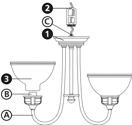
Drawing 2 - Fixture Assembly
