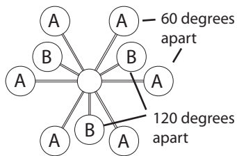
Drawing 2 - Fixture Assembly
