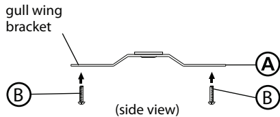
Drawing 2 - Fixture Mounting
