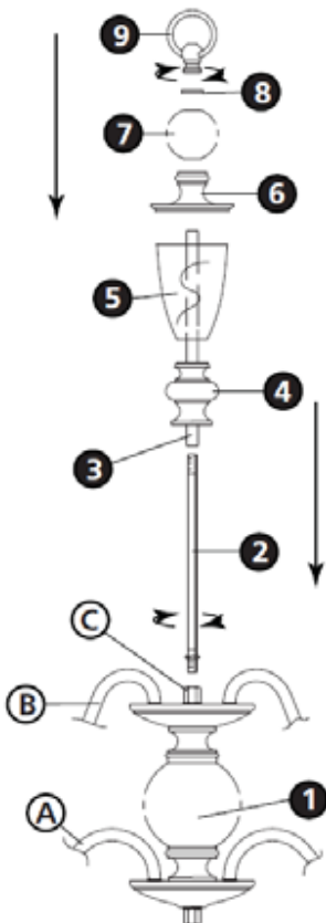
Drawing 2 – Fixture Assembly
