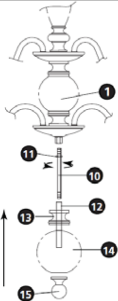
Drawing 1 – Bottom Assembly
