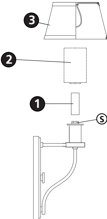
Drawing 2 - Shade Installation
