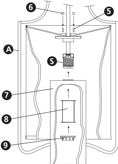
Drawing 2 - Shade mounting
