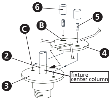
Drawing 3 - Arm Rotation
