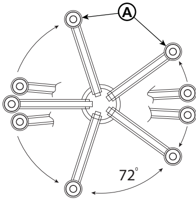
Drawing 1 - Assembly
