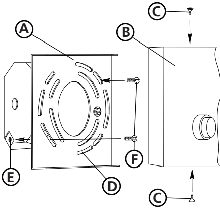
Drawing 1 - Fixture Mounting
