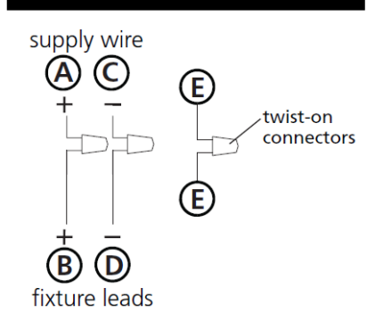
Drawing 3 – Post-Mount
