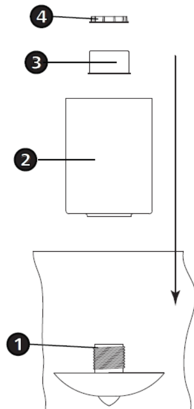
Drawing 2 – Glass Installation
