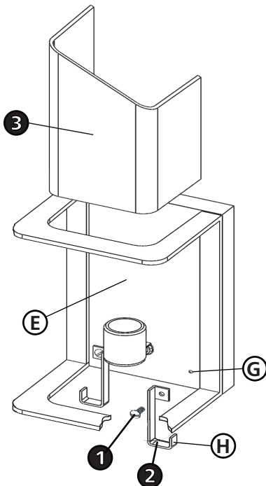
Drawing 2 - Fixture Mounting
