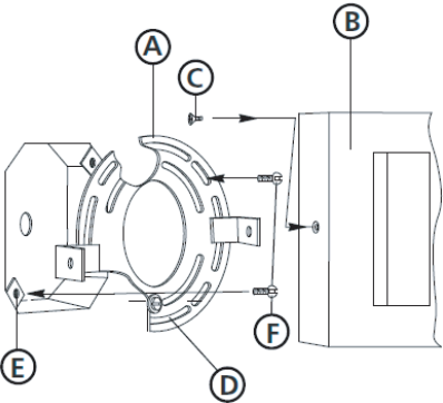
Drawing 1 – Fixture Mounting
