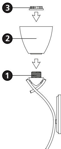
Drawing 3 - Fixture Assembly
