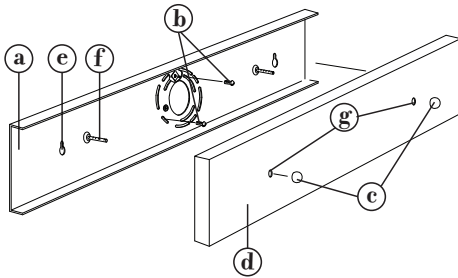
Drawing 2 - Bulb shield installation
