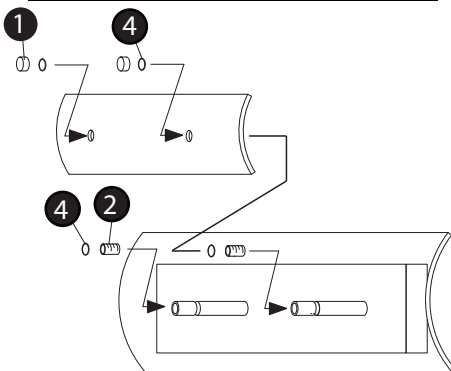
Drawing 4 - Glass installation
