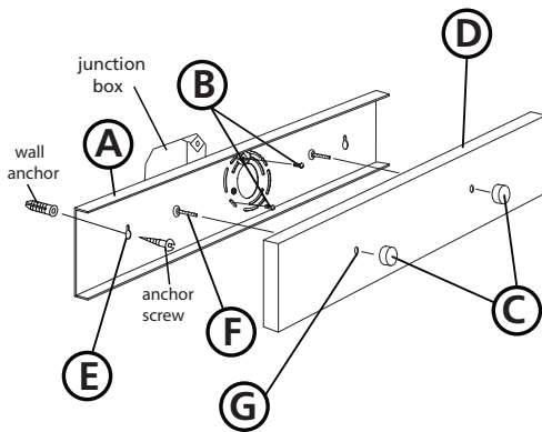
Drawing 1 - Mounting Detail
