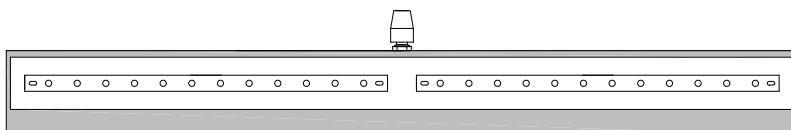
BTLEDR14" shade 1.6 Watt, 44 Lumen LED Backplate: 4 1/2" x 3 1/2"
