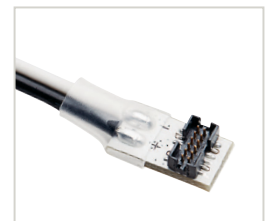
8T1TWRSWH Tape-to-Supply Lead 72" – 18AWG
