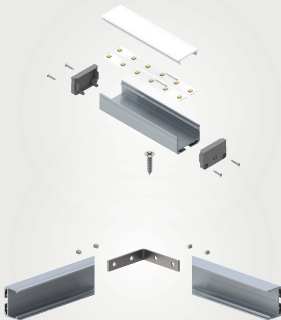
EXPLODED VIEW
