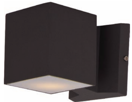
86107 ABZ, AL 2-Light Wall Sconce 4"W x 4"H x 5.75"Ext. 2 x 4.5W LED (Included) 630 Lumens
