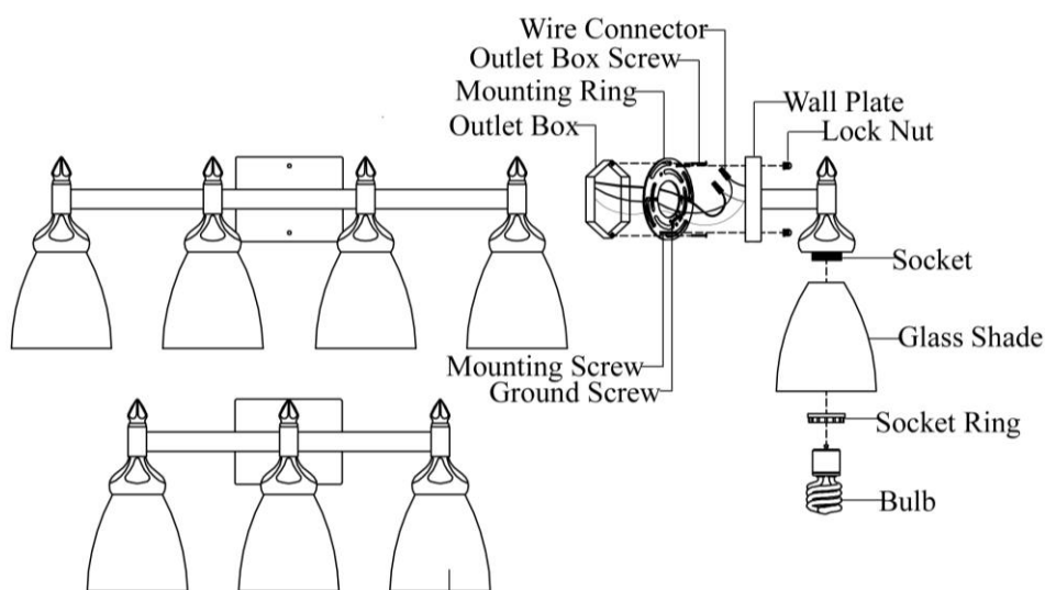
Fig.1: Install For Downward
