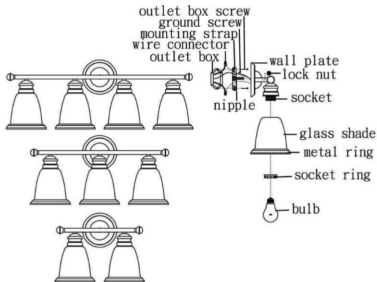
Fig. 1. Install for downwards
