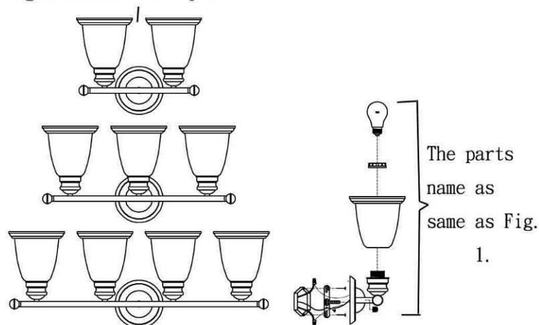
Fig. 2. Install for upwards
