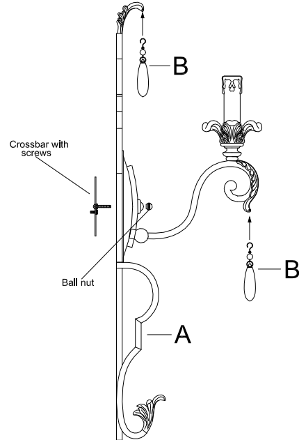
Side view of fixture
