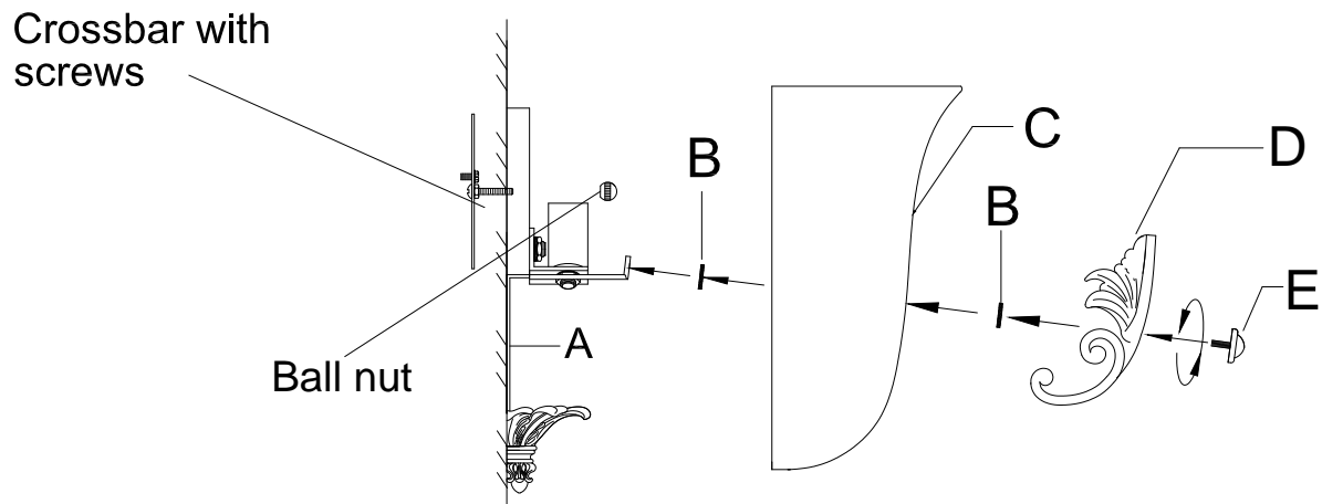
Side view of fixture
