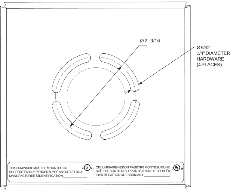
PLAN VIEW OF MOUNTING BRACKET
