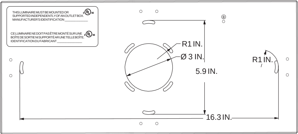
PLAN VIEW OF MOUNTING BRACKET
