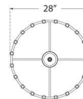
Vertical Top View (1:2)
