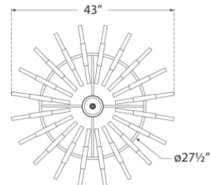
Horizontal Top View (1:2)
