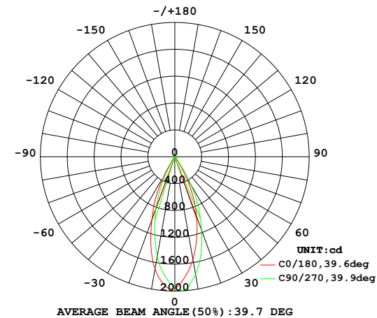
32° Beam Angle - 4500K
