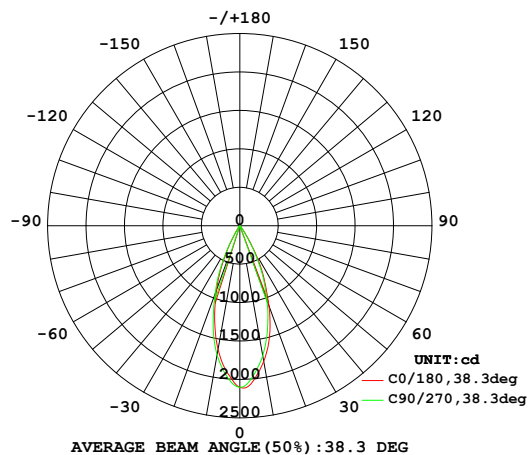
32° Beam Angle - 3500K
